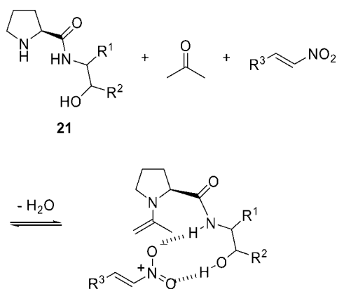
Scheme 2. L-Prolinamide-derived bifunctional organocatalysts.
