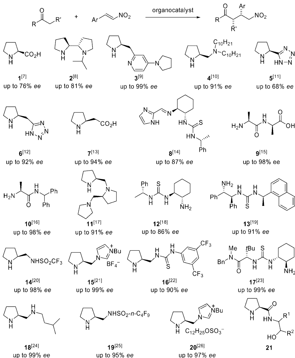
Scheme 1. Enantioselective conjugate addition of ketones to trans - \beta -nitrostyrene.
