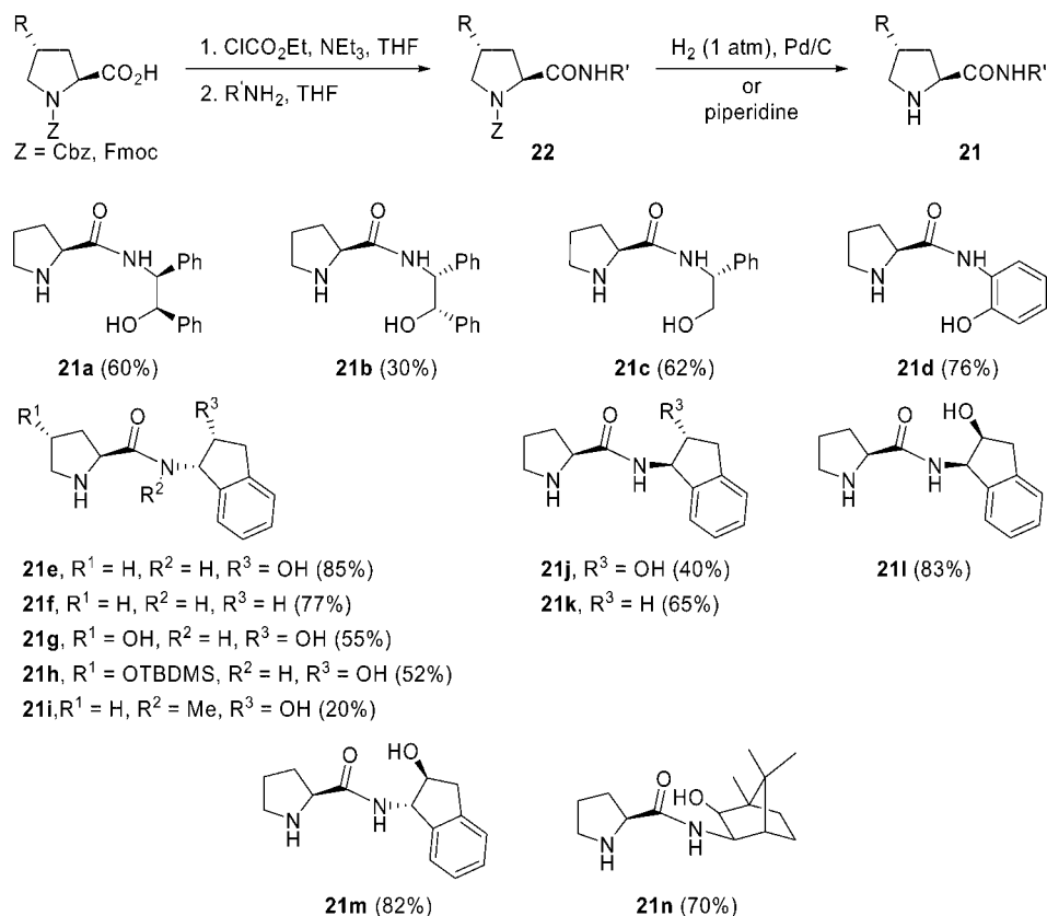
Scheme 3. Synthesis of bifunctional organocatalysts 21a–n .
