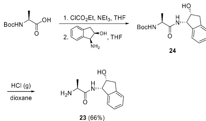
Scheme 4. Synthesis of bifunctional organocatalyst 23 .
