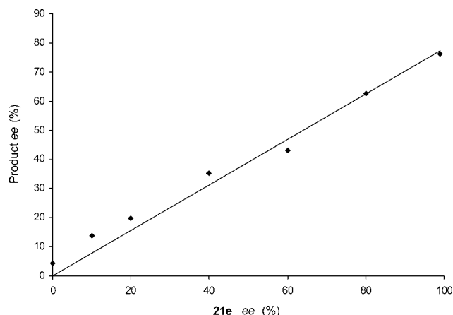
Figure 4. Observation of the linear relationship between the ee of 21e and that of 27aa .
