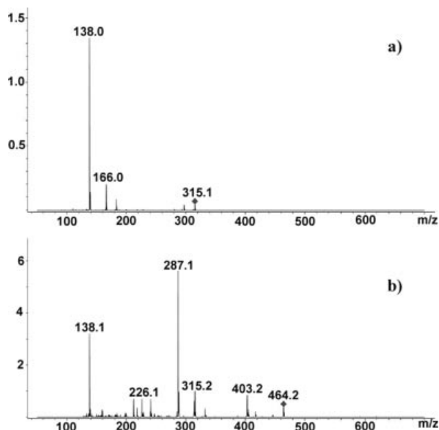
Figure 3. ESI-MS(+) spectra of the intermediates a) I · \text{H}^+ , b) II ^+ (see Scheme 8).
