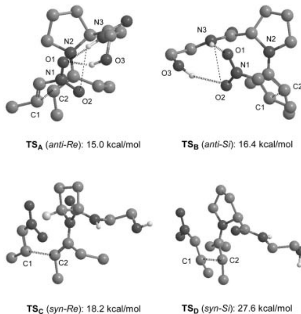
Figure 6. Transition-state geometries and activation energies for the reaction between 25a and 32 , calculated at B3LYP/6-31G* level.
