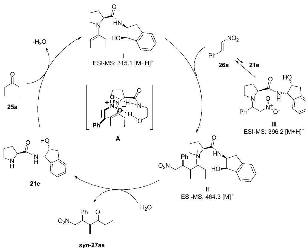
Scheme 8. Proposed mechanism for the 21e -catalyzed Michael addition.
