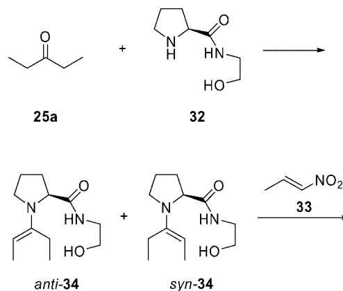
Figure 5. Model reaction used for the DFT computational studies.
