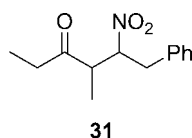
Figure 2. Regioisomeric product obtained in non-polar solvents.
