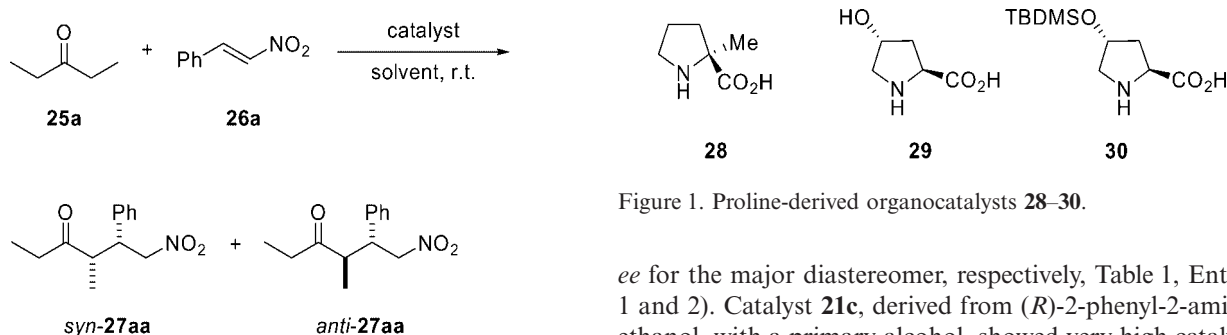
Scheme 5. Michael addition between 3-pentanone and trans - \beta -nitrostyrene.
