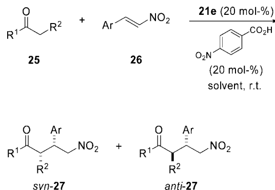
Scheme 6. Michael addition of ketones to \beta -nitrostyrenes.
