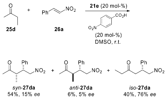
Scheme 7. Michael addition of butanone to trans - \beta -nitrostyrene.
